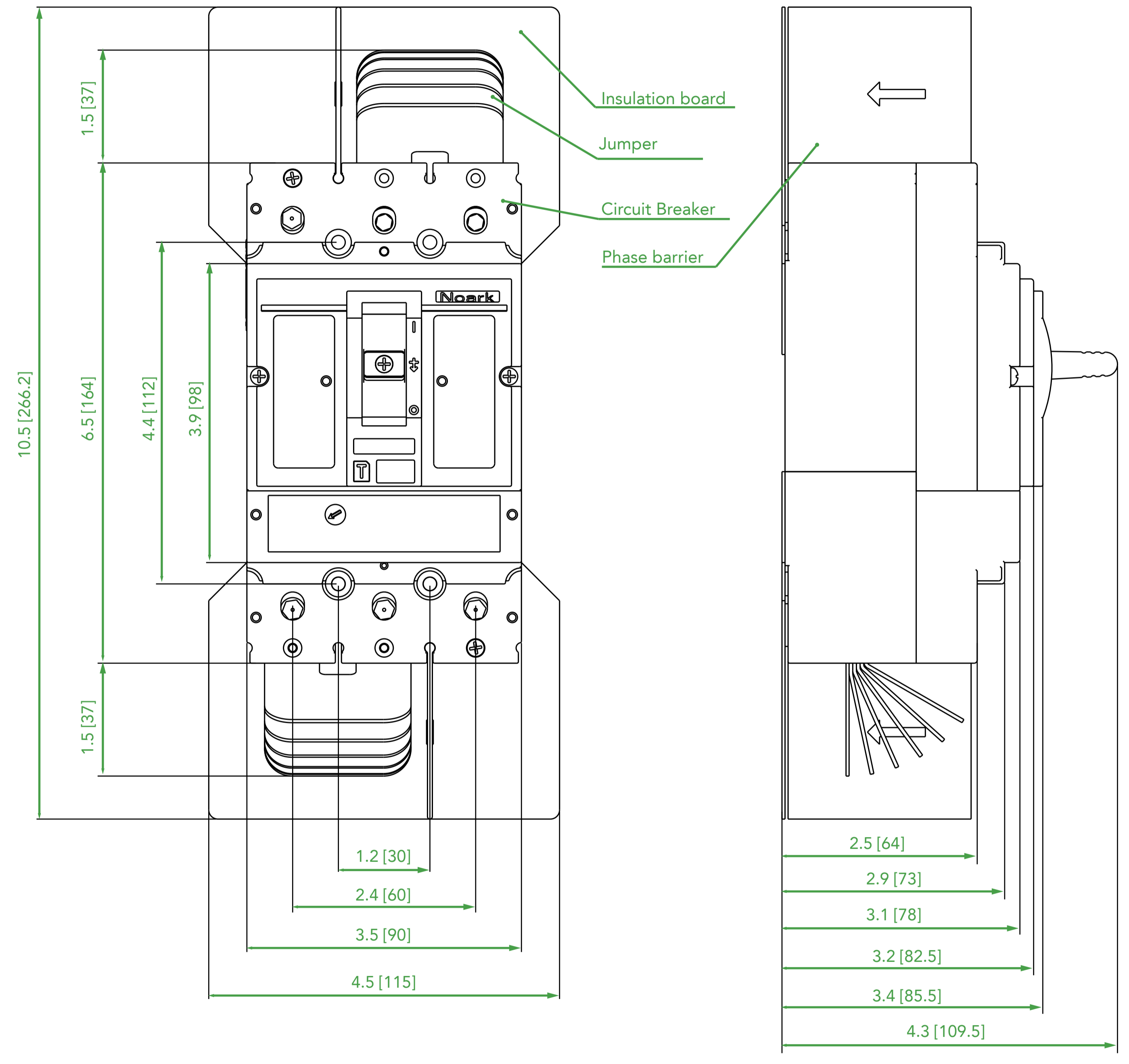
connection D
